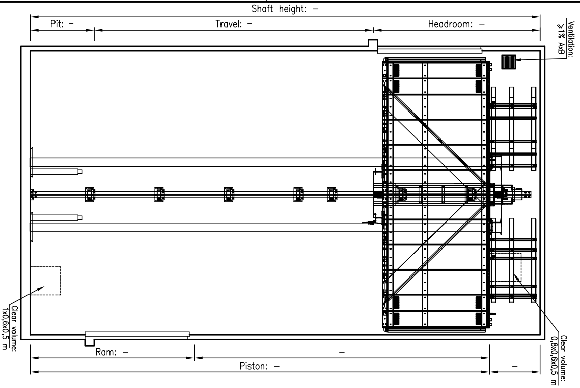
VERTICAL SECTION
