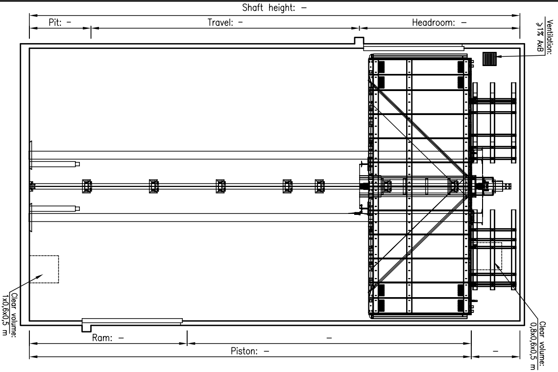
VERTICAL SECTION
